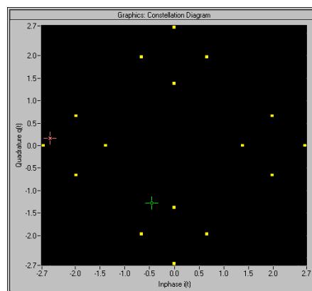
Fig.10 Constellation diagram of the signal without clipping, shows the level mapping
